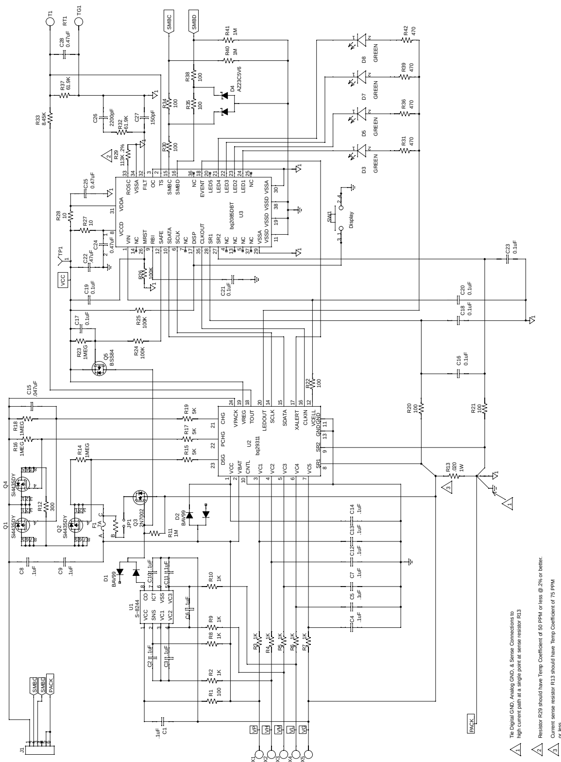
Figure 10. Typical bq2085-V1P2 Implementation
